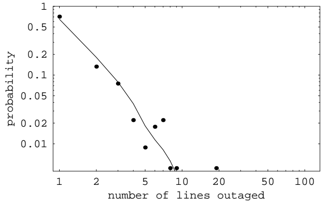
Fig. 3. Distribution of total number of outages Y estimated using branching process (line) and from data (dots); this log-log plot shows a heavy tail.
