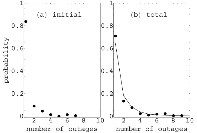
Fig. 2. Probability distributions of number of outages. (a) Initial outages Z_0 from data; (b) Total number of outages Y estimated using branching process (line) and from data (dots).
