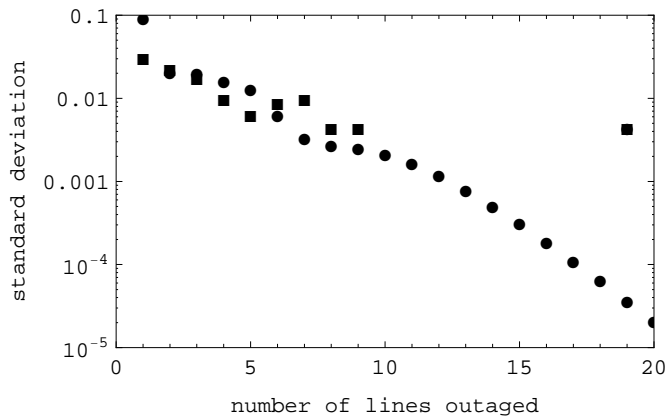
Fig. 4. Standard deviation \sigma_B for estimation via the branching process with one year of cascade data (circles) compared to the standard deviation \sigma_E for empirical estimation with 9 years of cascade data (squares). \sigma_B < \sigma_E for more than 5 line outages.
