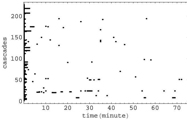
Fig. 1. Time since start of cascade for outages in each of the 226 cascades. The first 75 minutes of each cascade are shown (3 cascades exceeded 75 minutes). Multiple outages at the same time are shown slightly displaced.
